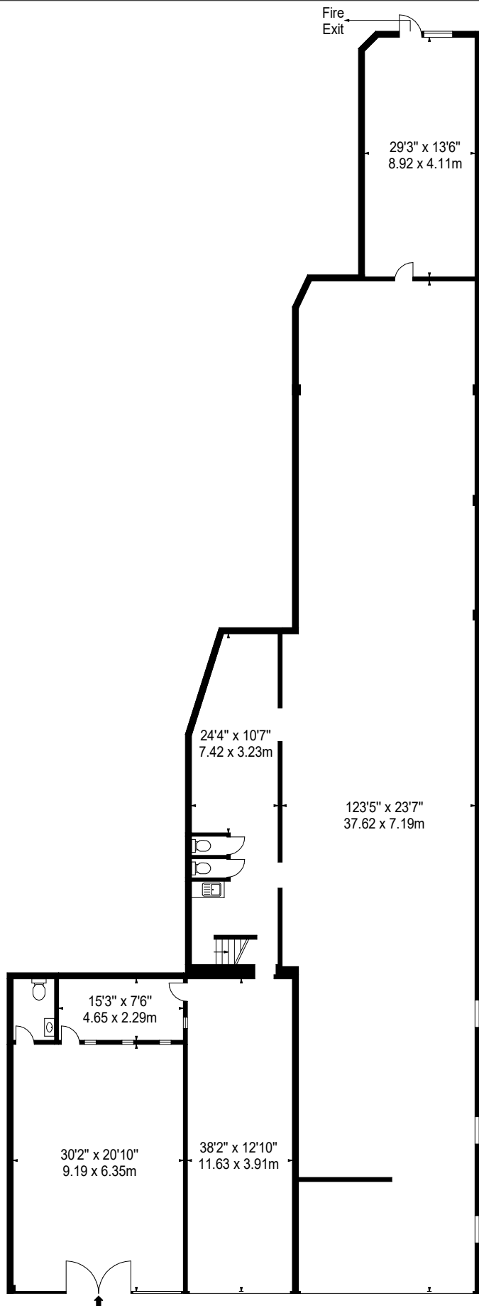
GROUND FLOOR
